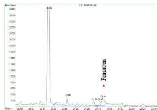
Figure 5. Chromatogram of phenanthrene in sediment samples after enlarged scale
